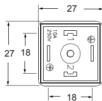
ISO DIN 43650 Form "A" Note: ISO connector available in 3+ Ground
