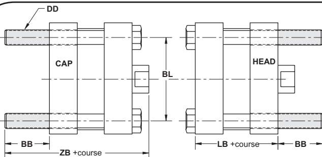
ST2X1 : Both tie rods extended ST2X2 : Cap end tie rods extended ST2X3 : Head end tie rods extended
