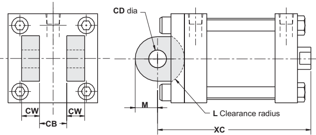
ST2P1 Detachable short clevis mount
