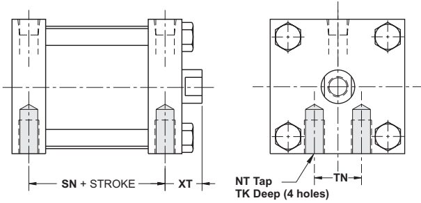
ST2S4 Bottom tap mount
