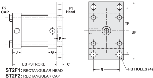
ST2F1 & ST2F2 Rectangular mounts
